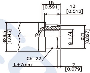
(4) G 1/4 FEMALE
