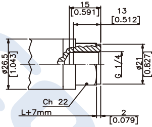
(4) G 1/4 FEMALE
